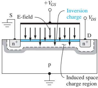
Figure 11.8 | Vertical electric field in an n-channel MOSFET.
